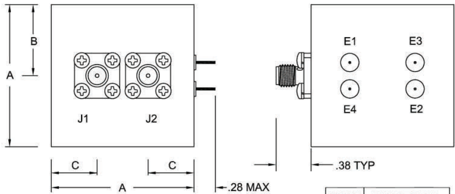
CASE DRAWING 21-018 / 21-019
